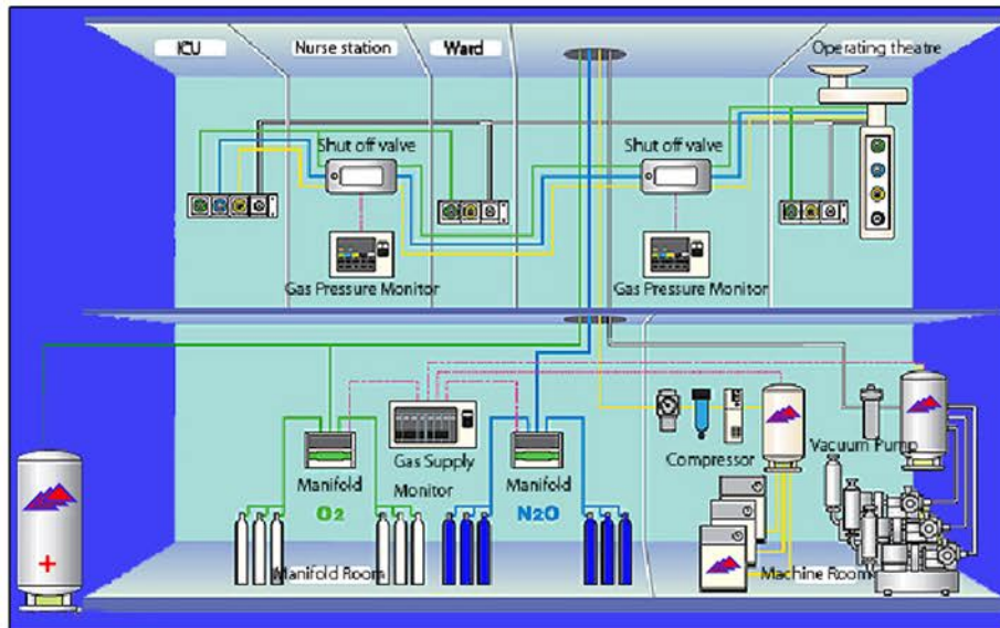
Flow Chart instalasi Gas Medis
